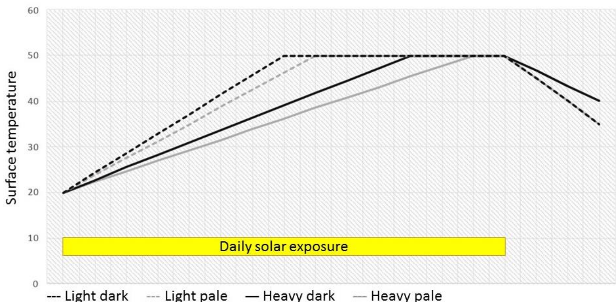
Figure 2 Surfaces temperature modification profile for the non-reflective families under heavy solar exposure.
